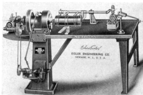
This tungsten wire-swaging machine with water circulating pump was a 1919 Eisler invention. The patent (No. 1,324,886) was assigned to Westinghouse.
